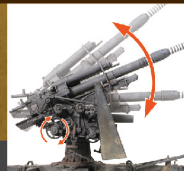
Flak gun elevates according to steering wheel movements (Via bevel gears mechanism)
